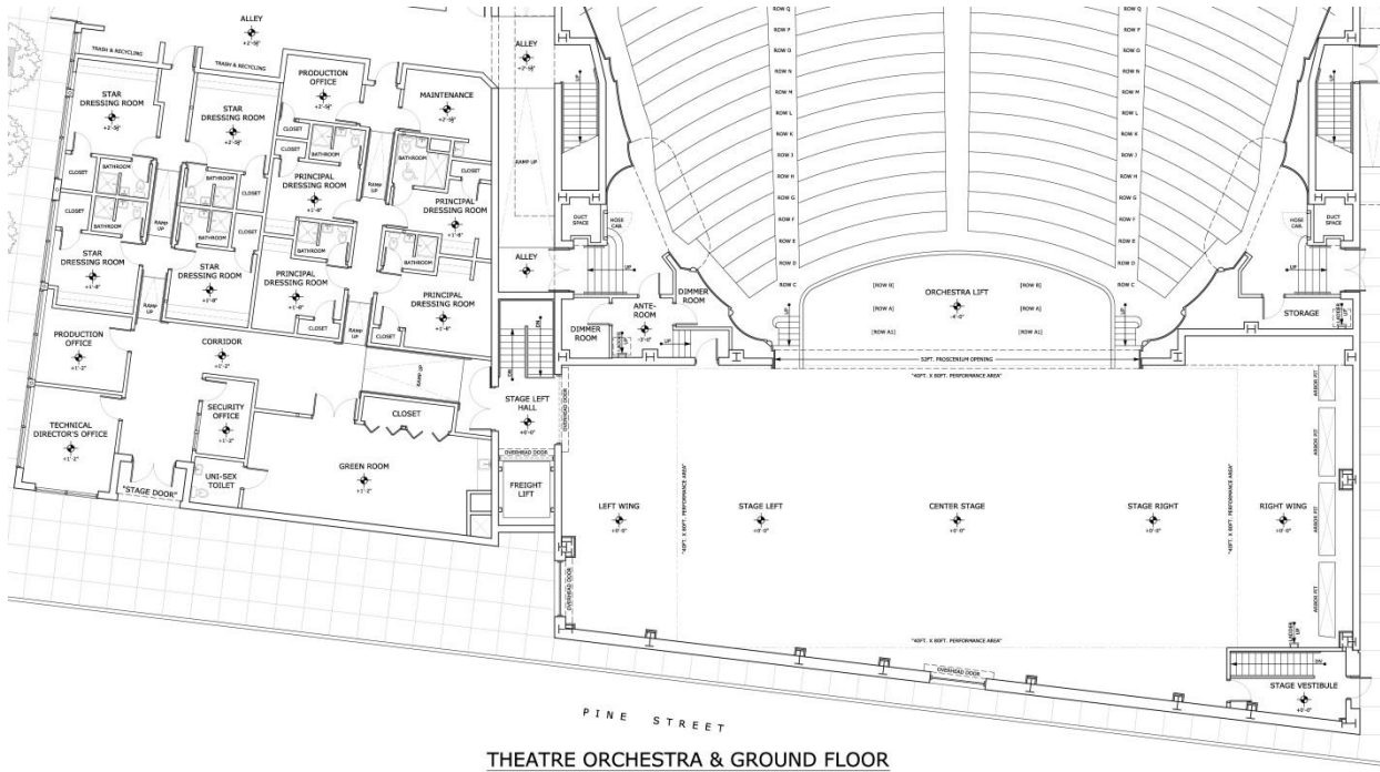
THEATRE ORCHESTRA & GROUND FLOOR
