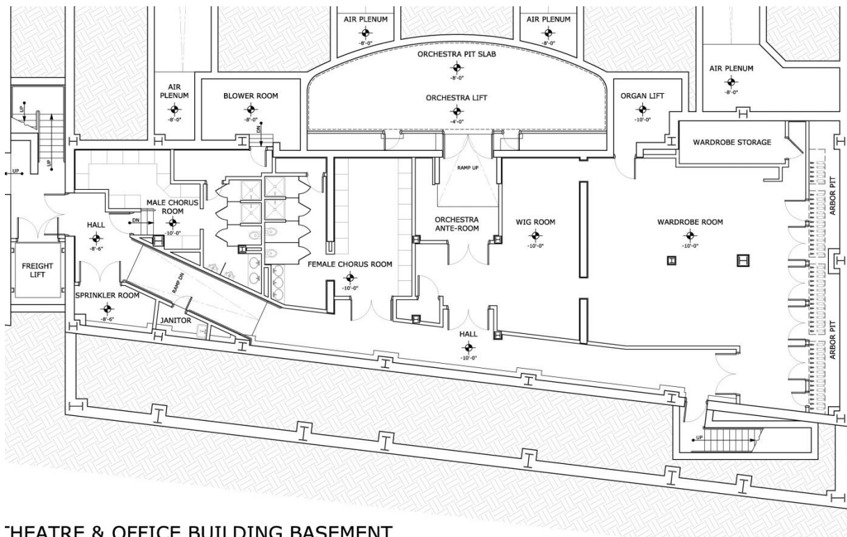
THEATRE & OFFICE BUILDING BASEMENT
